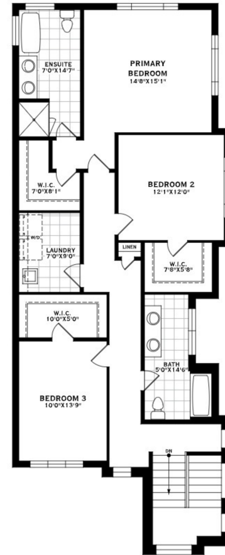
Second Floor
