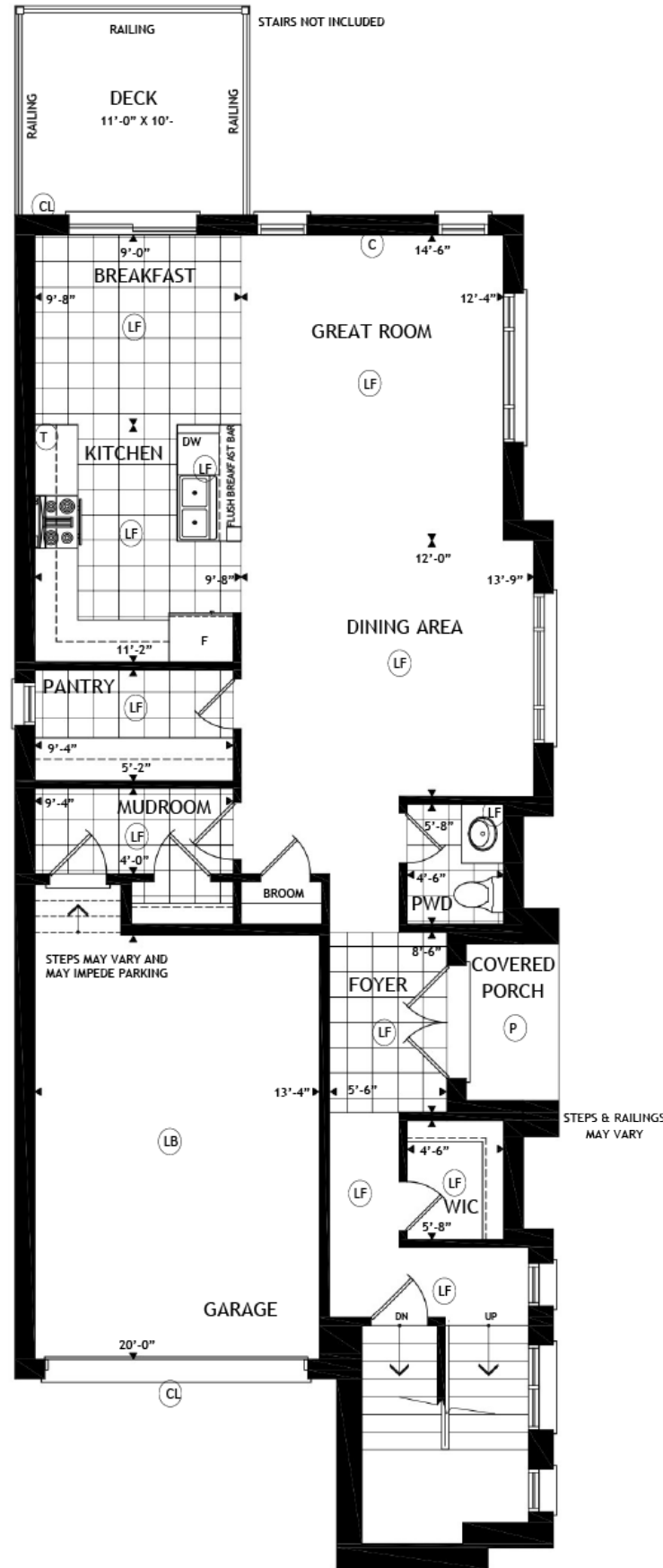
Main Floor
