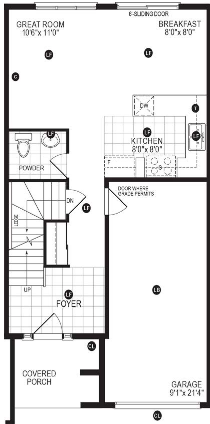
Main Floor
