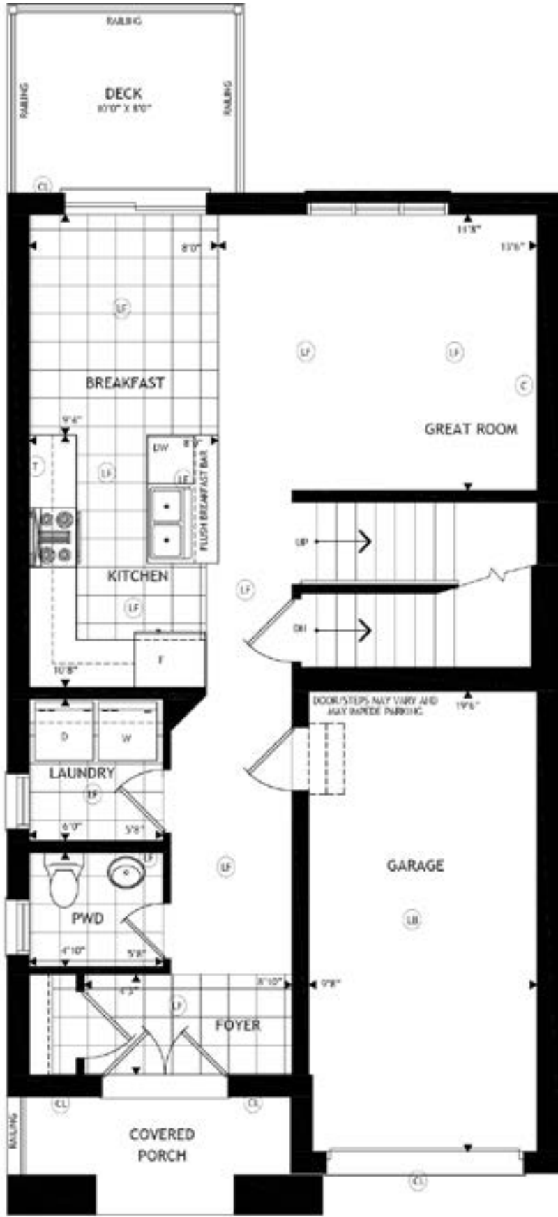
Main Floor
