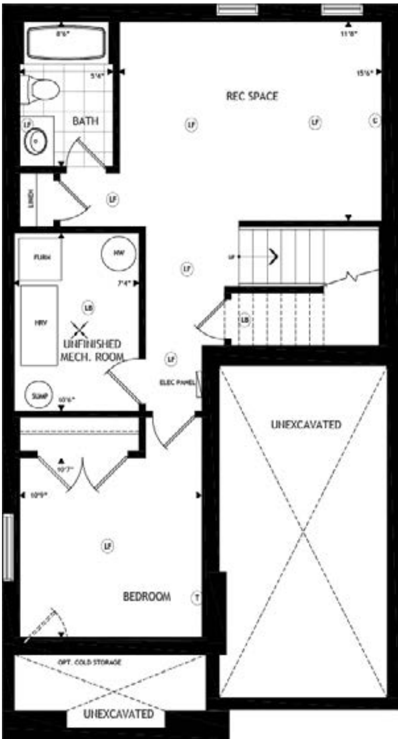
Finished Basement
