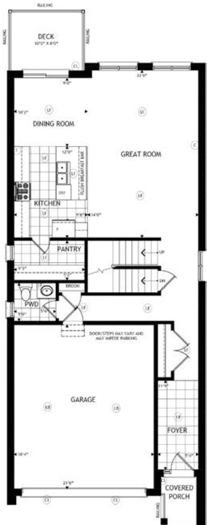
Main Floor
