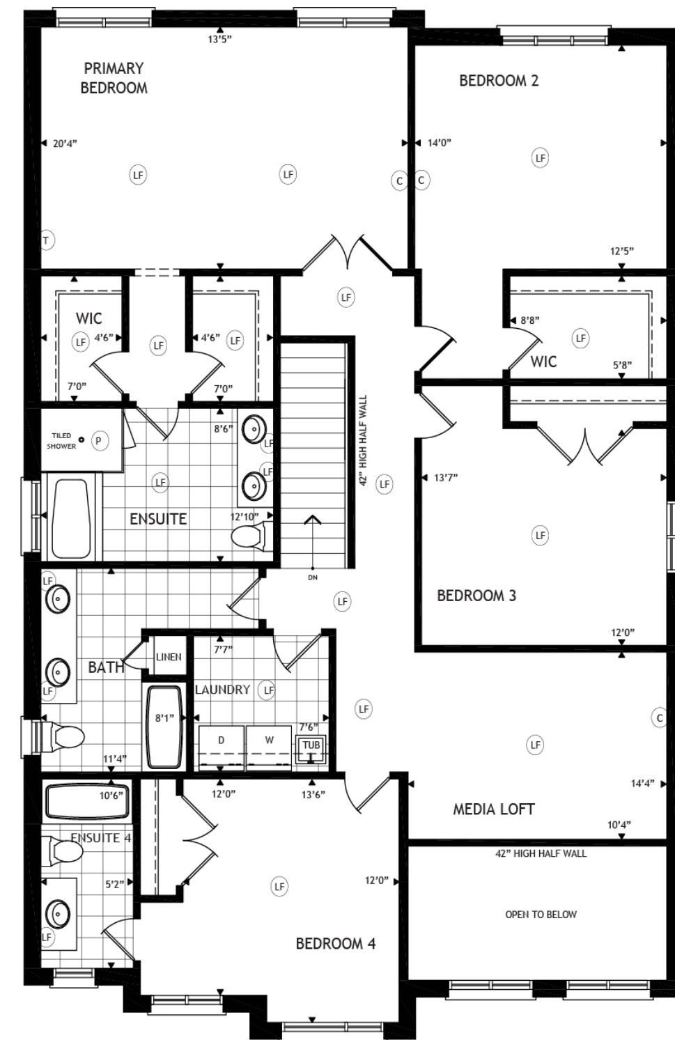
Primary Suite Second Floor
