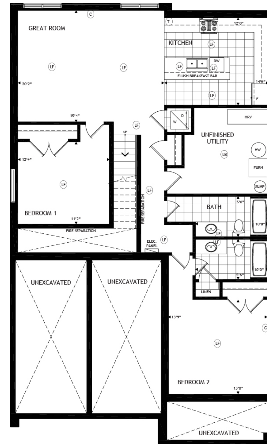
Secondary Suite Two Bedroom Basement
